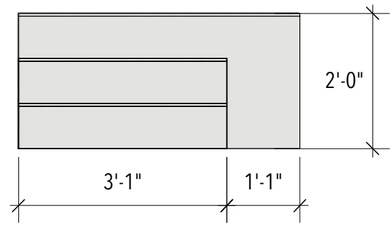
A-1 platform 1: front
