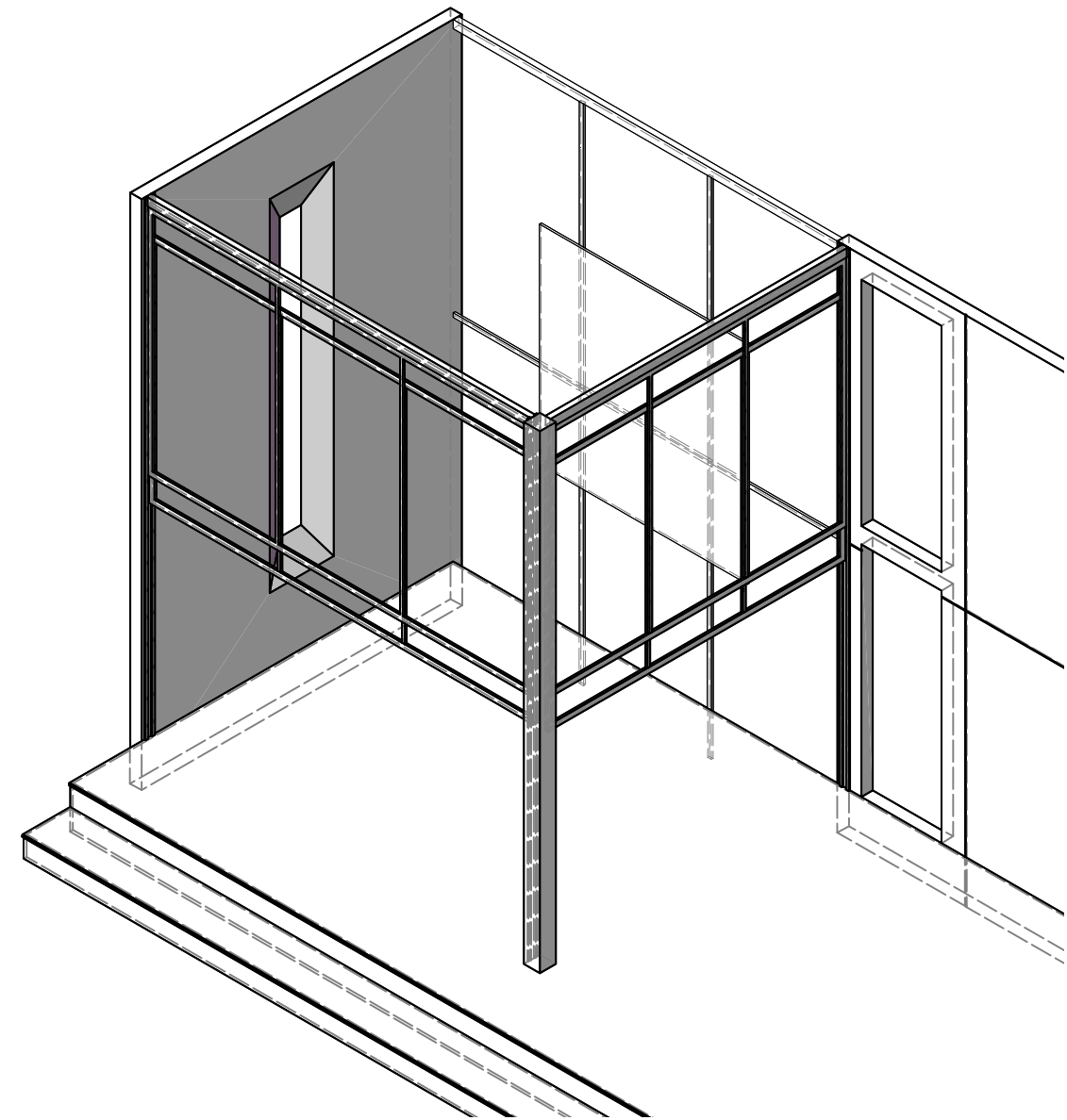
F-5 terrace window: isometric Scale: 1/4" = 1'-0"
