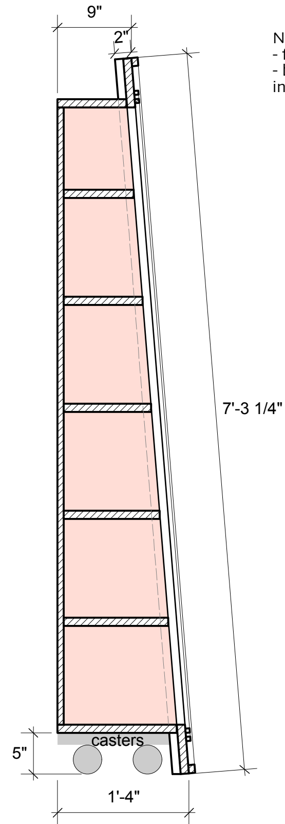
1 Section view
