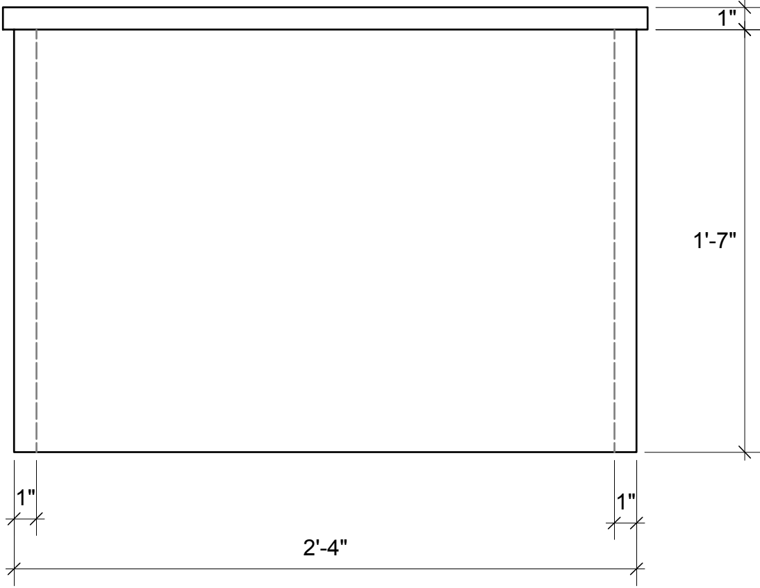
12-A Piano chair: front
