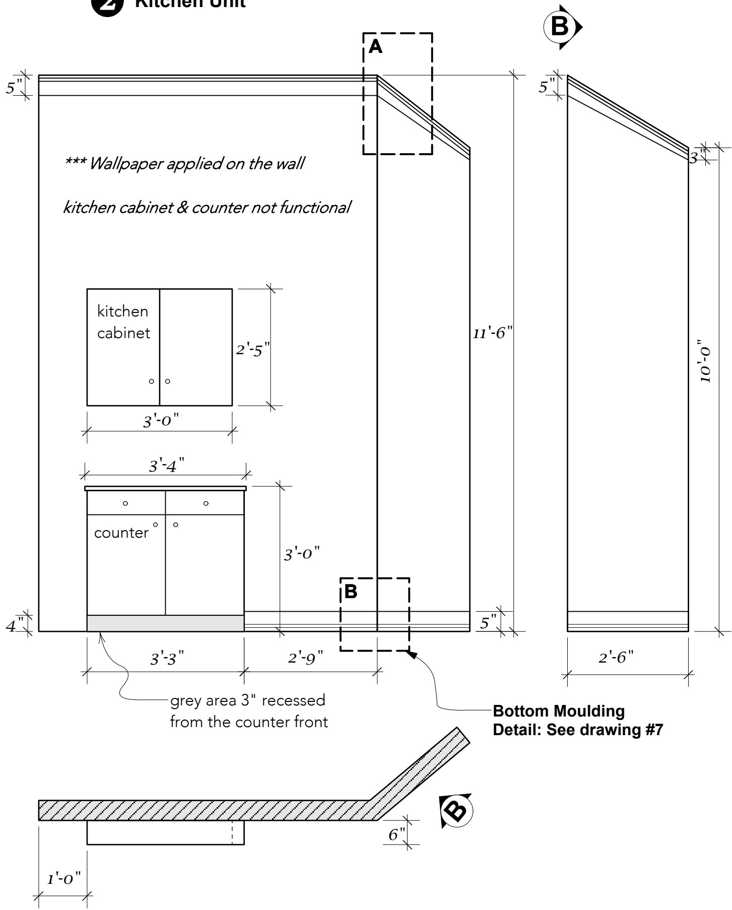
A. Kitchen Unit Crown Moulding Detail Scale: 1'=1'-0" (actual scale)
