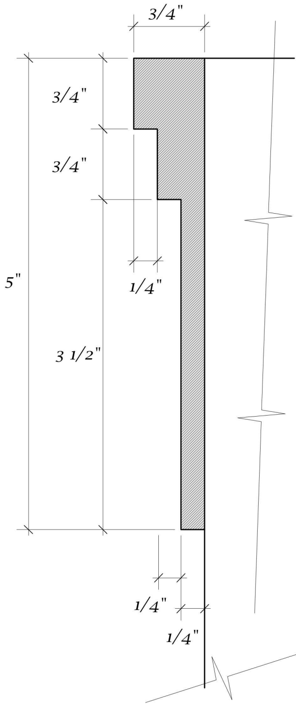
AA' Crown Moulding Section Detail Scale: 1'= 1'-0" (actual scale)
